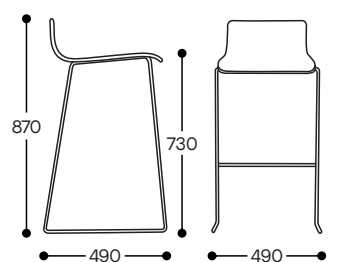
Stool with Sled Base (730 SH)
