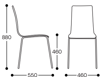
Chair with 4-Leg Base
