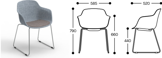
Tub shell with sled base (shown upholstered with seat pad)
