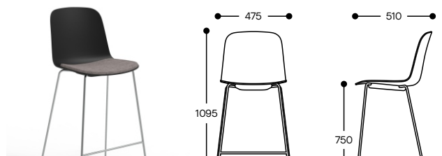
Standard shell with stool sled base (shown with seat pad)
