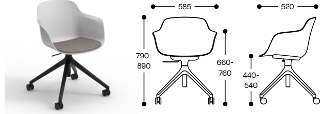
Tub shell with swivel base (shown with seat pad)
