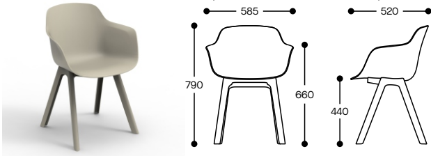
Tub shell sustainable eco chair (indent - extended lead time)
