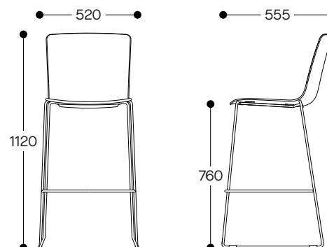
SLED HIGH STOOL
