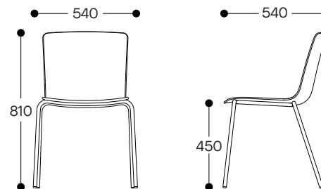
4-LEG STEEL CHAIR
