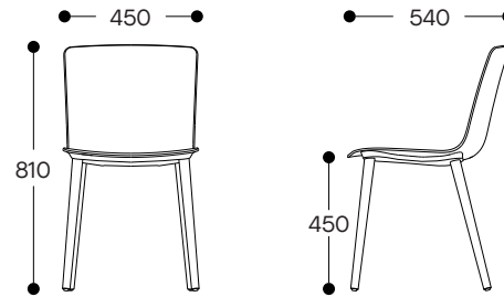
4-LEG TIMBER CHAIR
