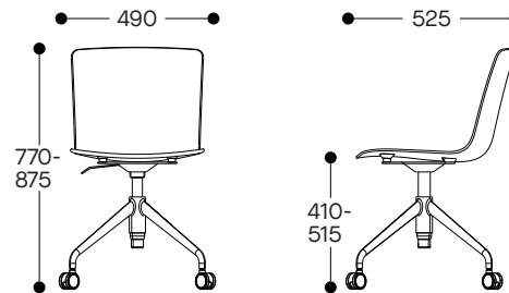
4-STAR CASTOR CHAIR
