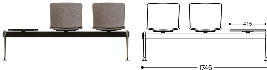
BEAM WITH 2 SEATS AND SIDE TABLE
